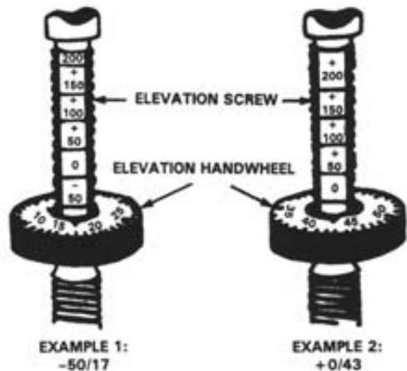
Figure 6-29. Elevation Reading.
