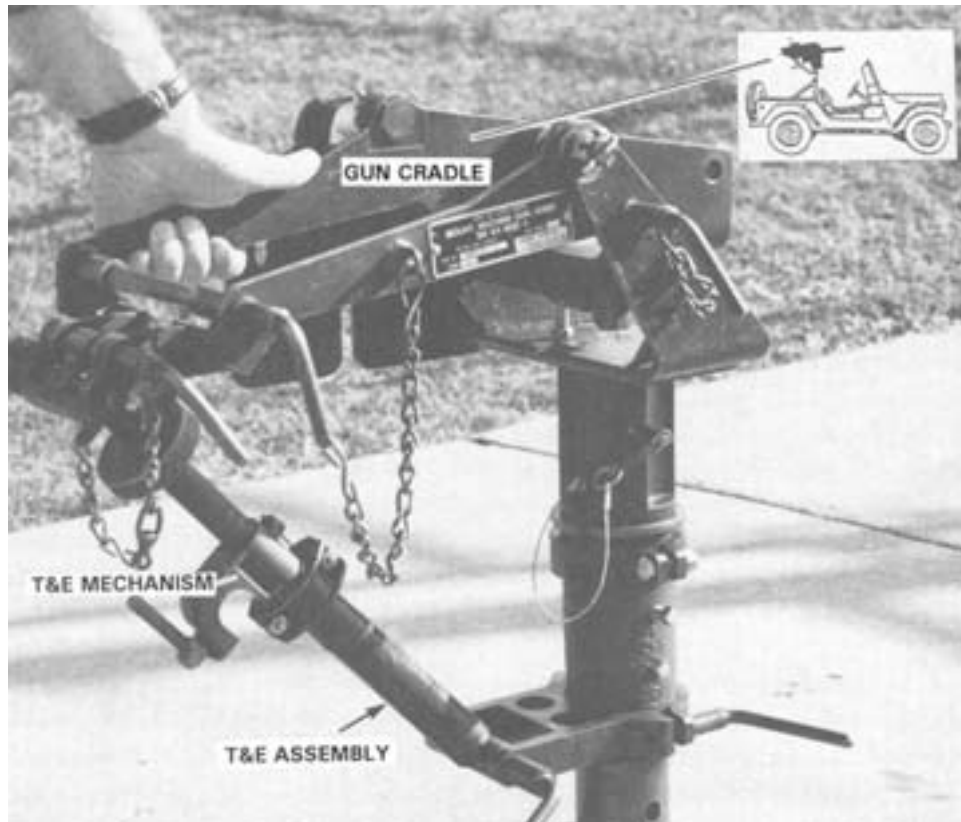
Figure 5-37. Pedestal Mount M4.
