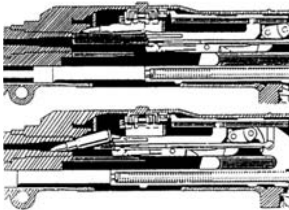
Figure 3-25. Chambering.
