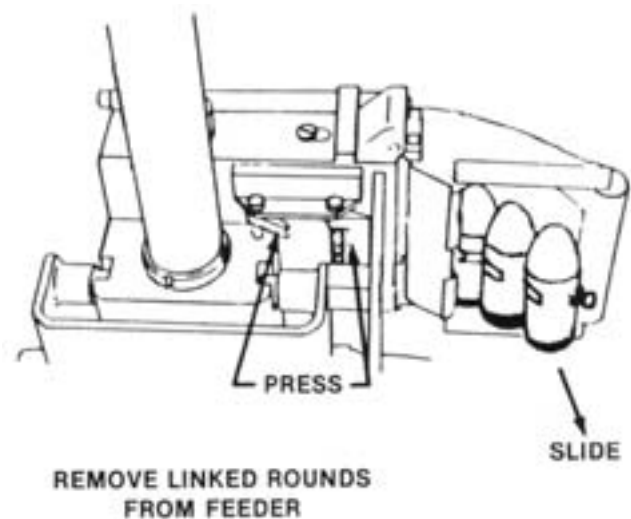
Figure 5-50. Clearing Rounds From Gun.
