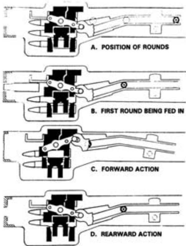
Figure 3-23. Feeding.
