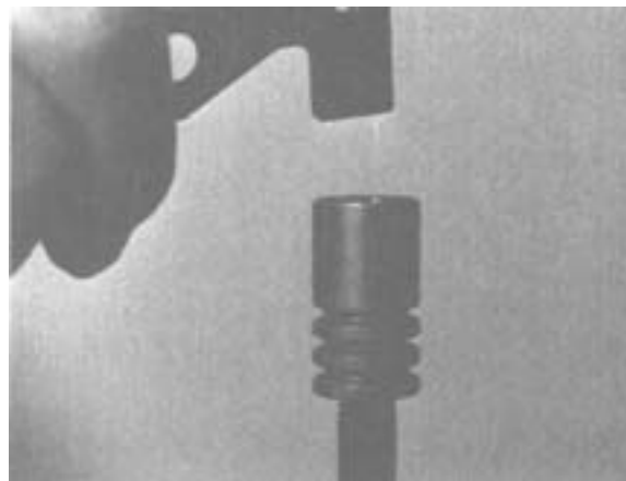
Figure 2-40. Cleaning the Hole in the Front of the Piston.
