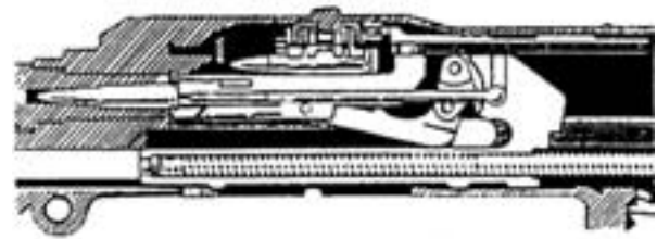
Figure 3-26. Locking.
