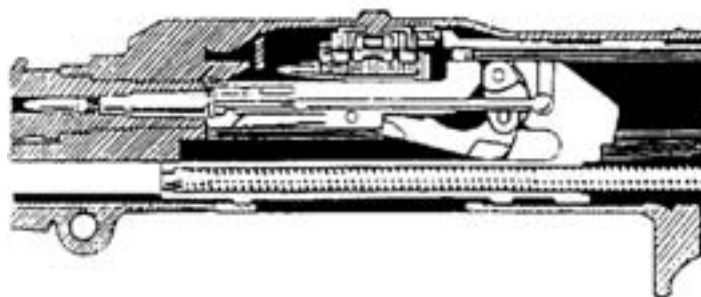
Figure 3-27. Firing.
