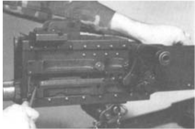
Figure 4-14. Removing the Barrel Buffer Group and Barrel Extension Group.
