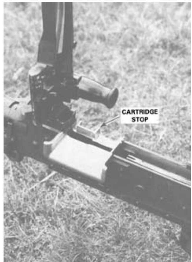
Figure 3-57. Feed Tray.
