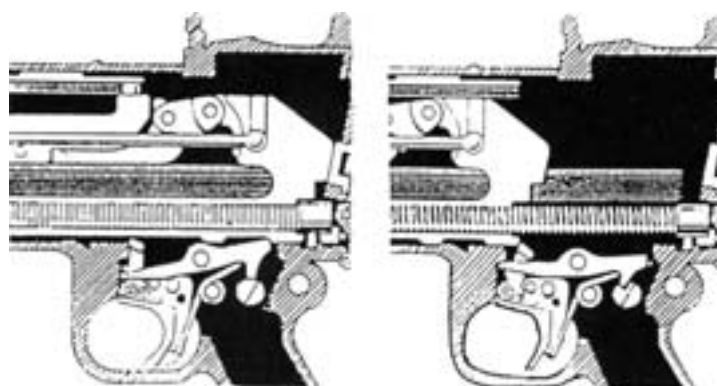
Figure 3-22. Trigger Pull Releasing the Operating Group.
