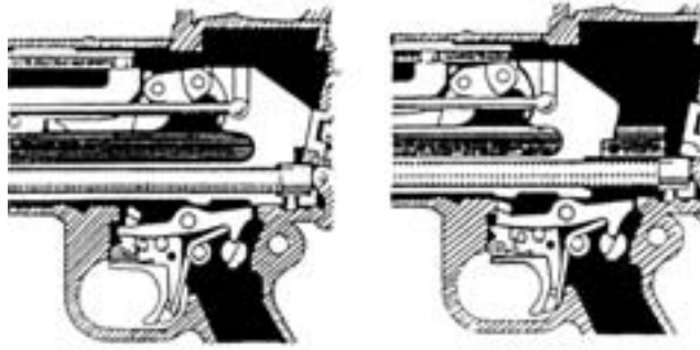
Figure 3-31. Cocking.
