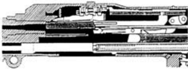
Figure 3-55. Firing From the Open Bolt Position.
