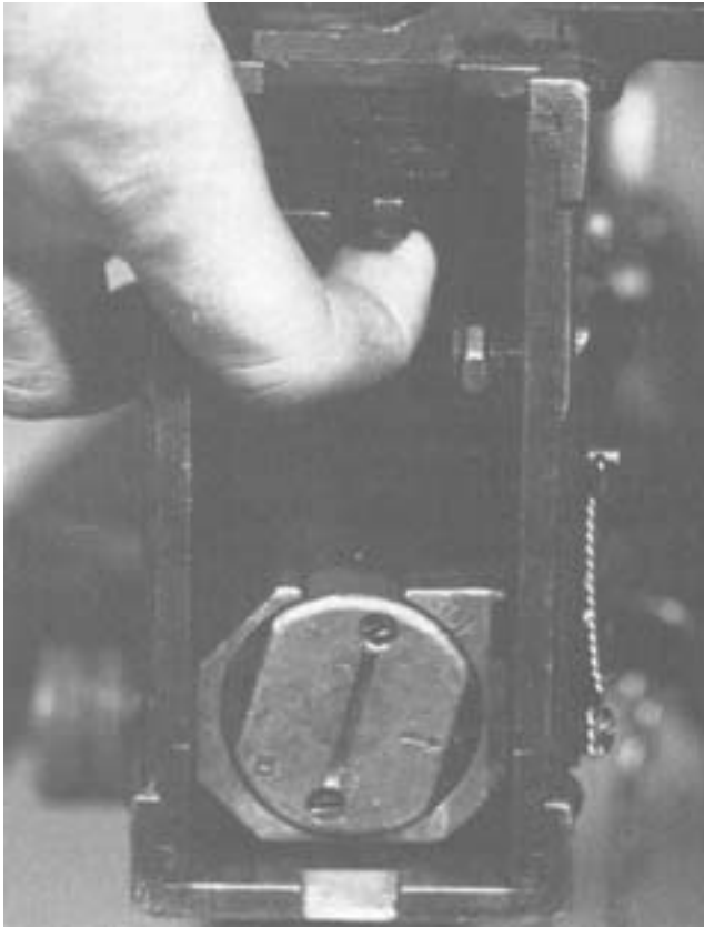
Figure 4-55. Depressing the Trigger.
